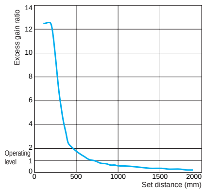
Convergent-reflective
