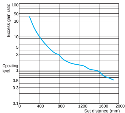
Diffuse-reflective
