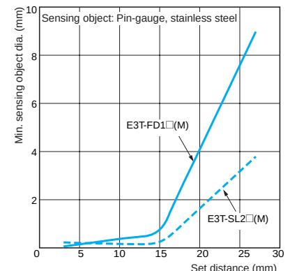
Diffuse-reflective
