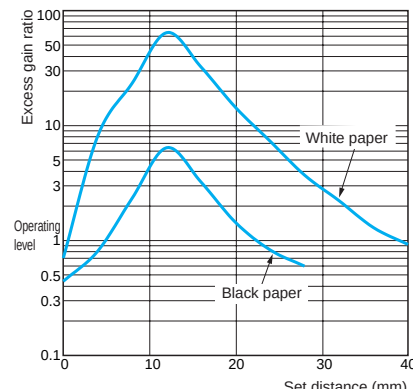
Sensing Distance vs. Material
