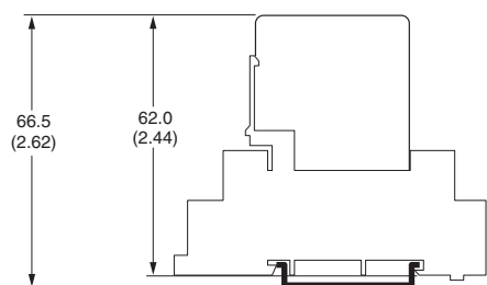
P2RF-□
