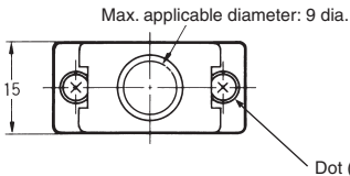
9-contact Hood
