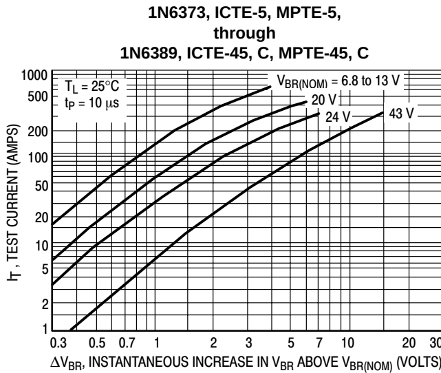
Figure 6. Dynamic Impedance
