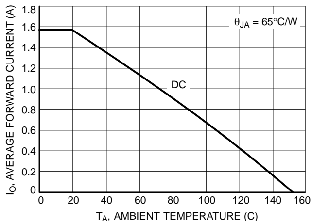
Figure 4. Current Derating
