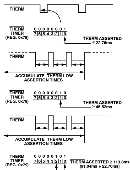
Figure 28. Understanding the THERM Timer
