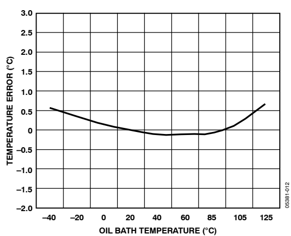
Figure 12. Remote Temperature Error vs. ADT7475 Temperature
