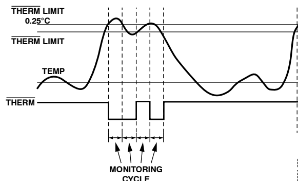
Figure 30. Asserting THERM as an Output, Based on Tripping THERM Limits
