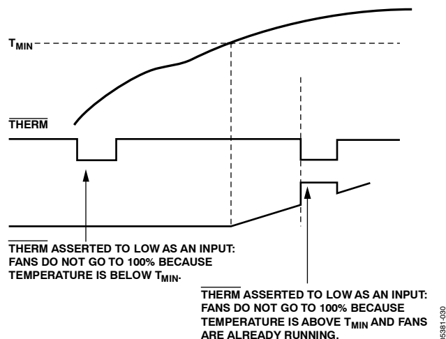
Figure 27. Asserting THERM Low as an Input in Automatic Fan Speed Control Mode
