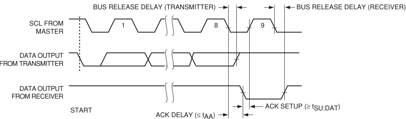
Figure 3. Acknowledge Timing
