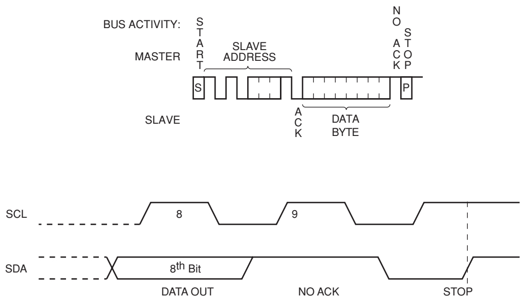
Figure 9. Immediate Read Sequence and Timing
