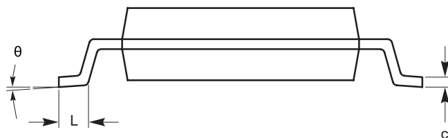
END VIEW
