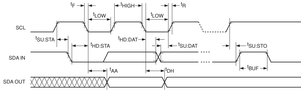
Figure 4. Bus Timing
