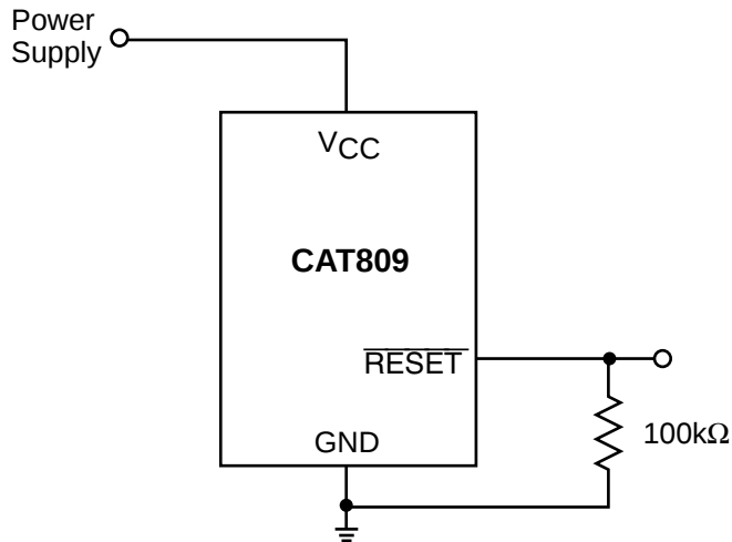
Figure 3. \overline{\text{RESET}} Valid with V_{CC} Under 1.0 V
