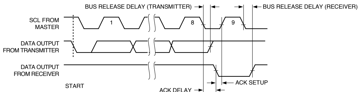
Figure 7. Acknowledge Timing
