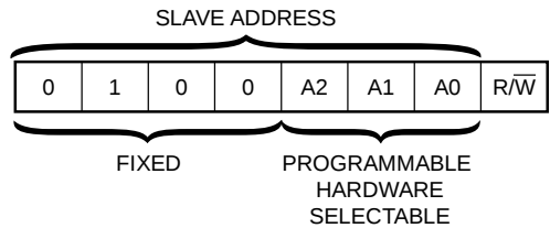
Figure 6. CAT9534 Slave Address
