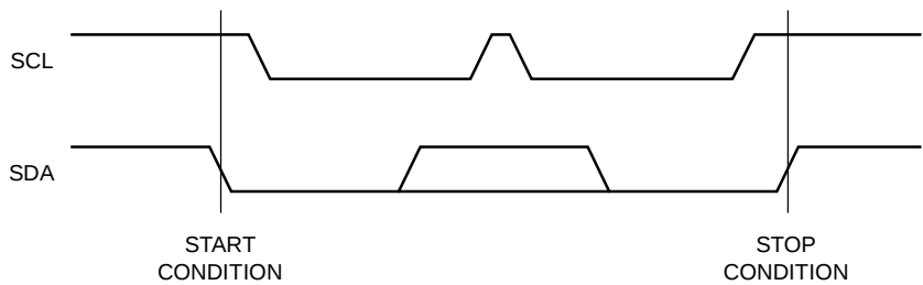
Figure 5. START/STOP Condition
