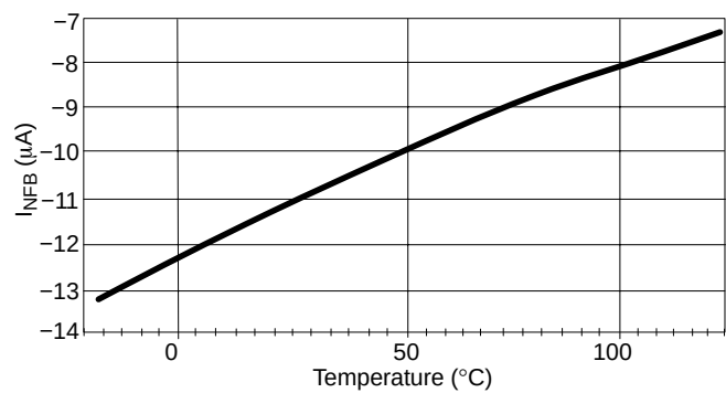
Figure 14. I_{NFB} vs. Temperature (CS5172/4 only)
