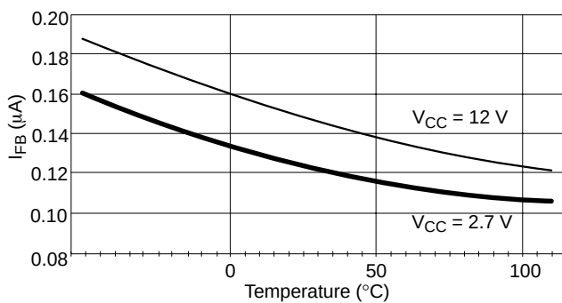
Figure 13. I_{FB} vs. Temperature (CS5171/3 only)
