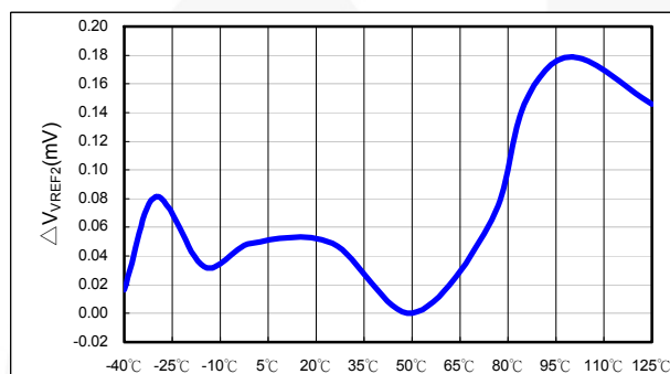
Figure 18. \Delta V_{VREF2} vs. Temperature
