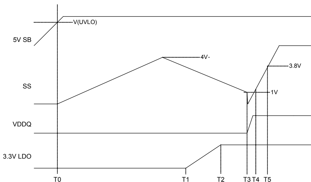
Figure 8. Start-up Sequence into S0
