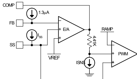
Figure 14. SS Clamp and FB Open Protection
