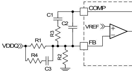
Figure 12. Compensation Network
