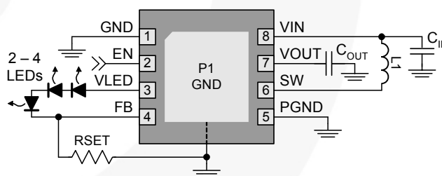
Figure 1. Typical Application
