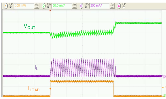
Figure 20. Load Transient 0mA to 150mA, V_{IN}=3.6V , t_{RISE}=t_{FALL}=100ns , 5μs/div.
