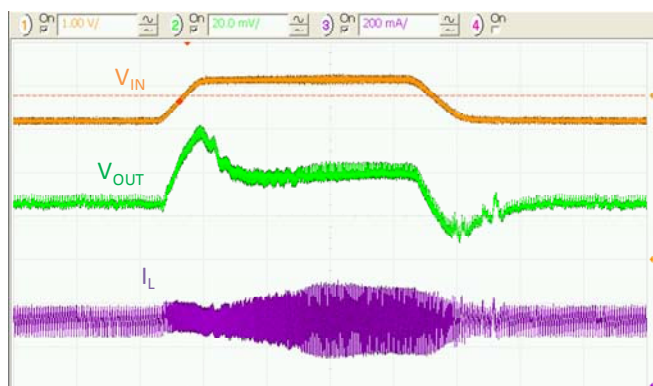
Figure 19. Line Transient at V_{IN}=3.2V to 4.2V , 300mA Load, t_{RISE}=t_{FALL}=10\mu s , 20μs/div.
