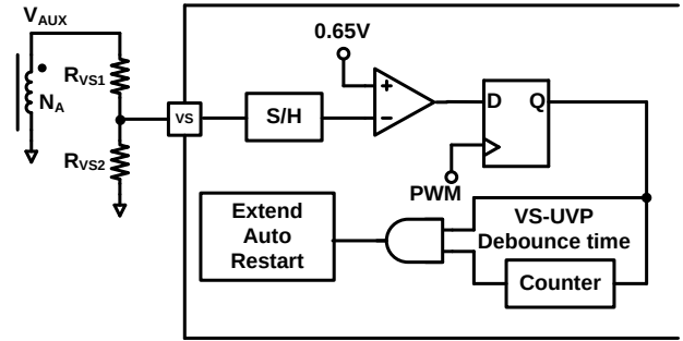
Figure 36 VS-UVLP Protection Circuit
