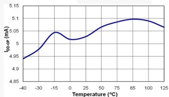
Figure 9. Operating Current
