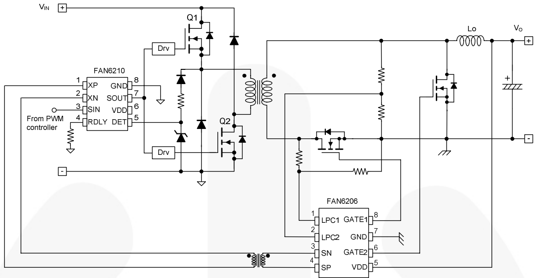
Figure 1. Typical Application
