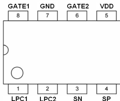
Figure 4. Pin Configuration
