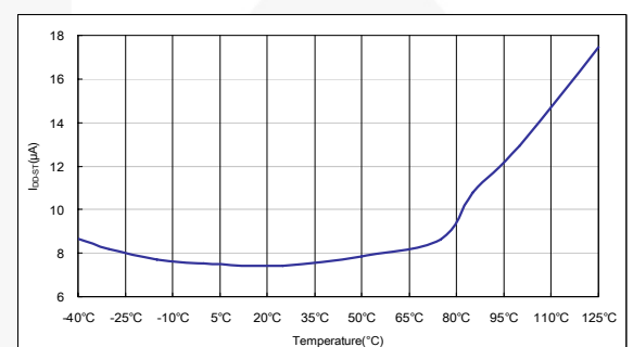
Figure 8. Startup Current
