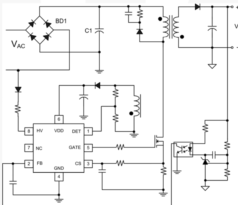
Figure 1. Typical Application
