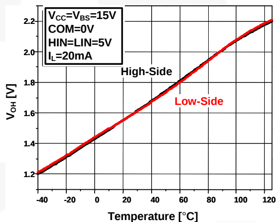
Figure 25. High-Level Output Voltage vs. Temp.
