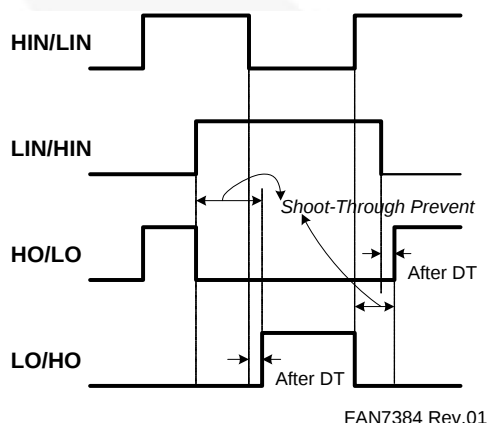
Figure 35. Waveforms for Shoot-Through Prevention
