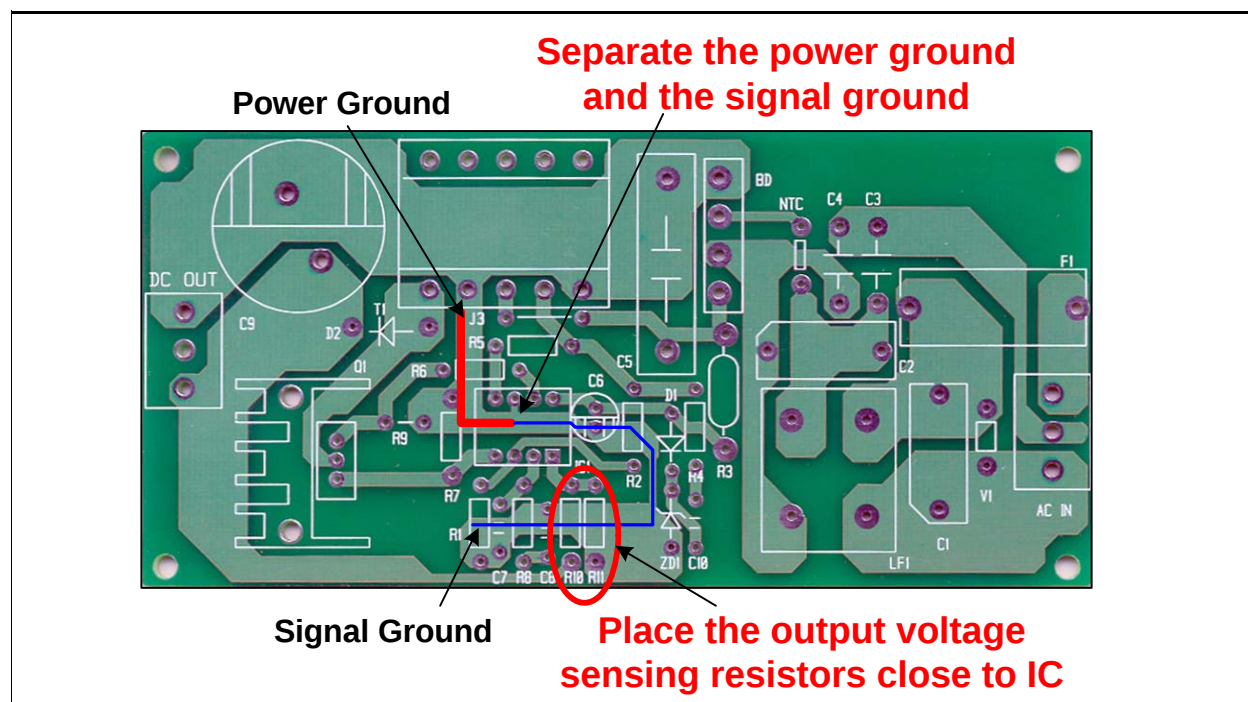
Figure 39. PCB Layout Considerations for FAN7530
