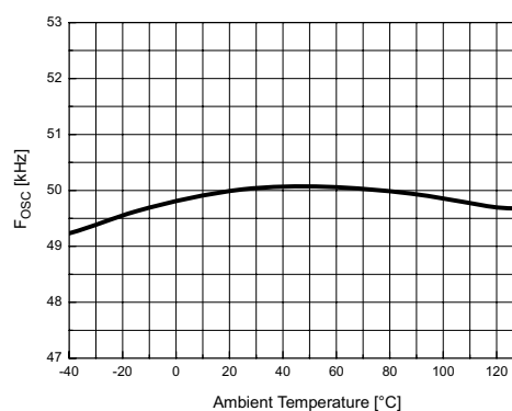
Figure 5. Operating Frequency vs. Temp.
