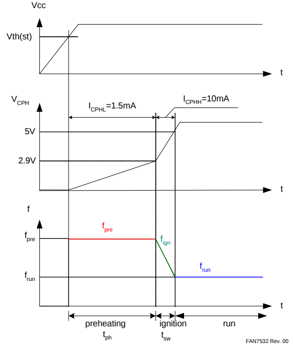
Figure 17. Operating Modes
