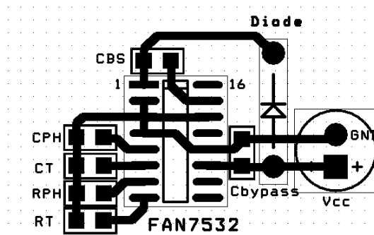
Figure 20. PCB Layout
