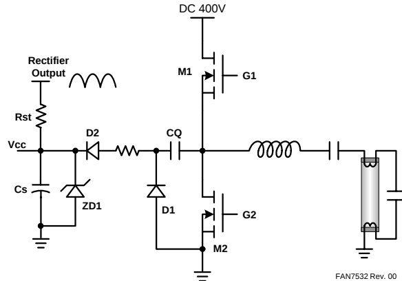
Figure 15. Start-up Circuit
