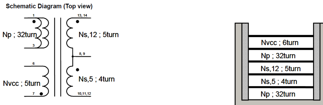
Figure 27. Transformer Specification
