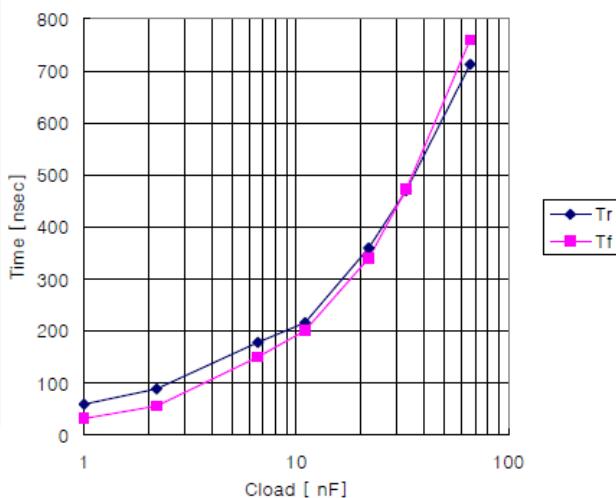
Figure 7. Cload vs. t_R & t_F
