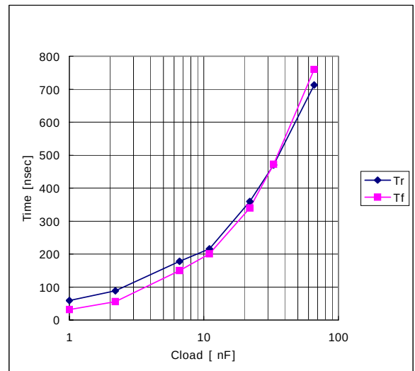
Figure 4. Cload vs. Tr & Tf
