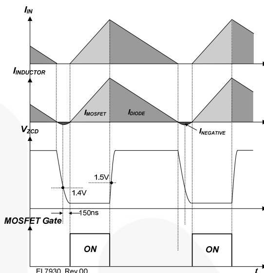
Figure 42. Input and Output Current Near Input Voltage Peak
