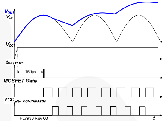
Figure 34. Restart Timer at Startup
