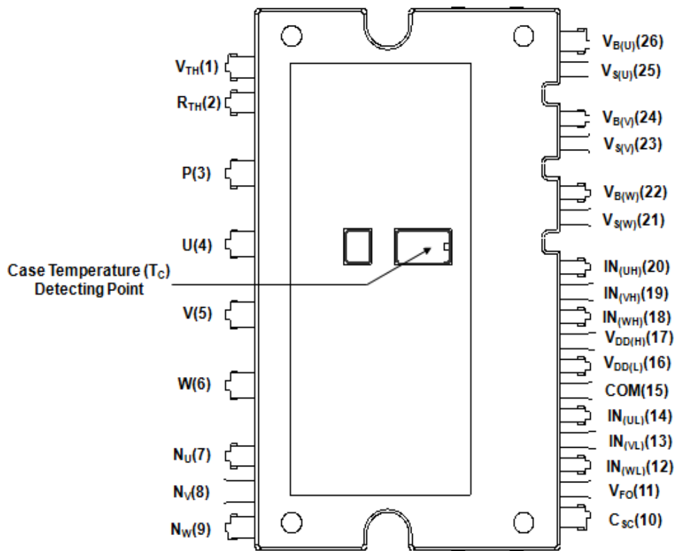
Figure 2. Top View
