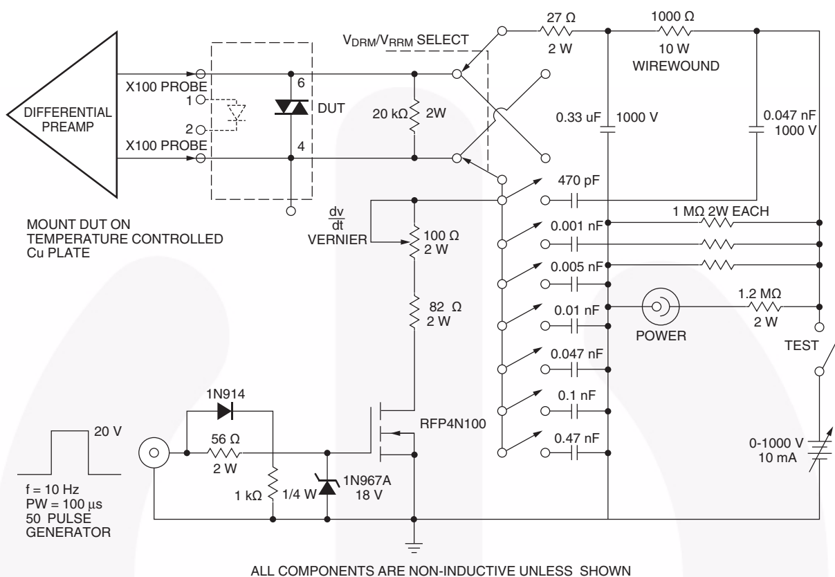
Figure 14. Circuit for Static \frac{dv}{dt} Measurement of Power Thyristors
