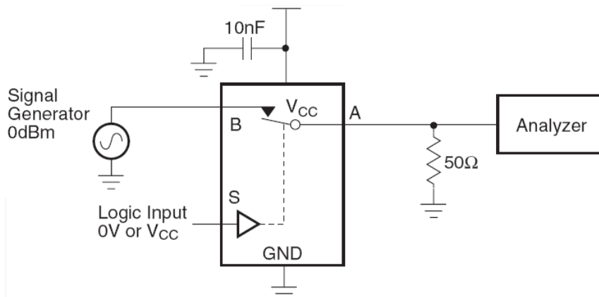
Figure 10. Bandwidth
