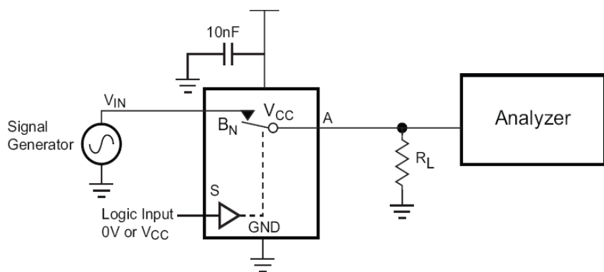
Figure 11. Harmonic Distortion
