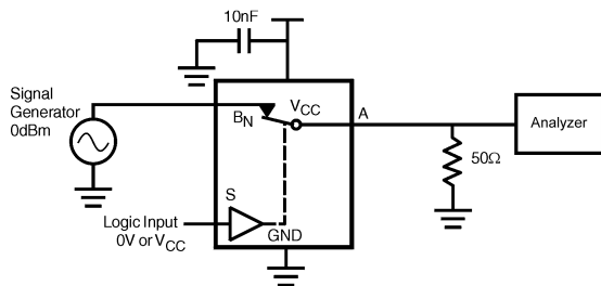
FIGURE 7. Bandwidth
