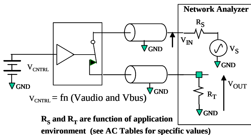
Figure 19. USB Bandwidth
