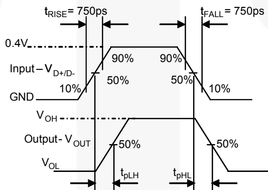
Figure 18. Pulse Skew: t_{SK(P)} = | t_{pHL} - t_{pLH} |
