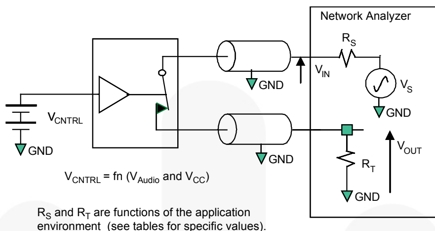
Figure 20. USB Bandwidth
