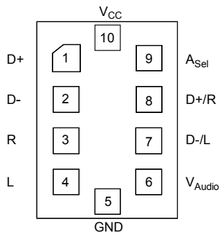
Figure 2. 10-Pin MicroPak™
