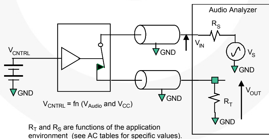
Figure 25. Total Harmonic Distortion
