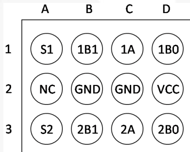
Figure 5. 12-Ball WLCSP (Bump Side View)
