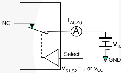
Figure 5. On Leakage
