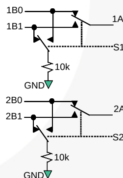
Figure 1. Analog Symbol
