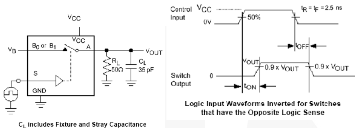
Figure 4. Turn-On / Turn-Off Timing
