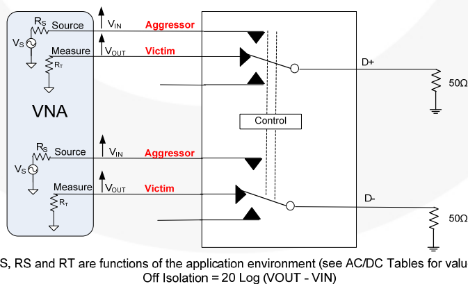
Figure 13. Non-Adjacent Channel-to-Channel Crosstalk (SDD21)
