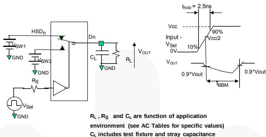
Figure 11. Break-Before-Make Interval Timing
