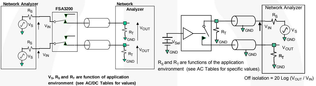
Figure 11. Insertion Loss
