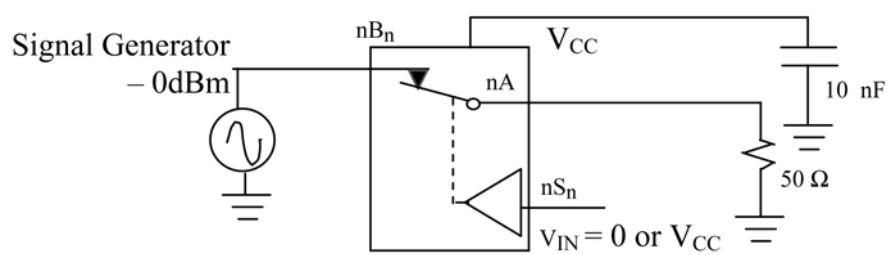
FIGURE 9. Bandwidth
