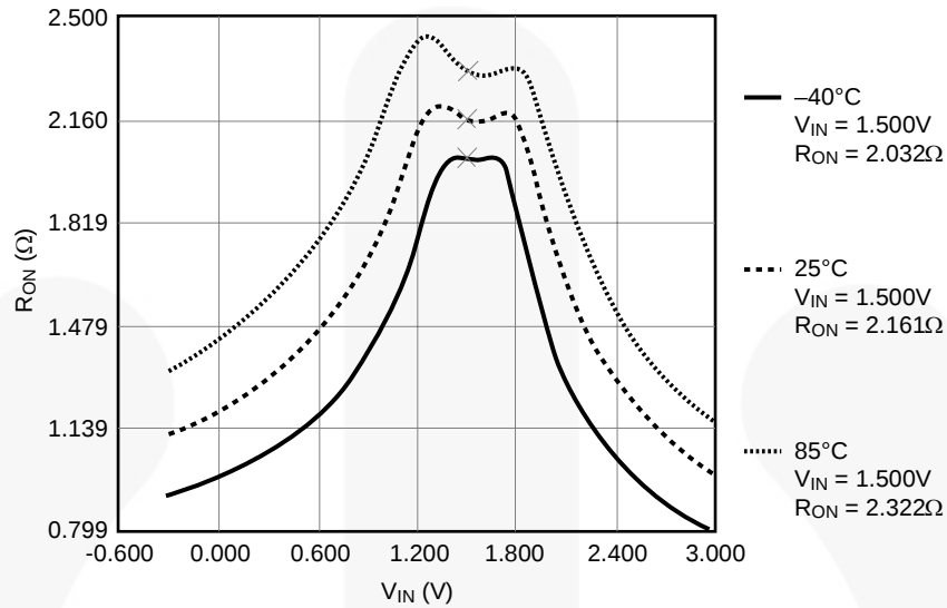
Figure 6. R_{ON} Switch On Resistance, I_{ON} = 100\text{mA} , V_{CC} = 2.7
