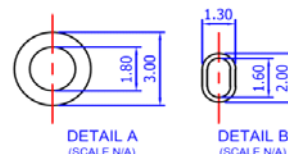
LAND PATTERN RECOMMENDATIONS
