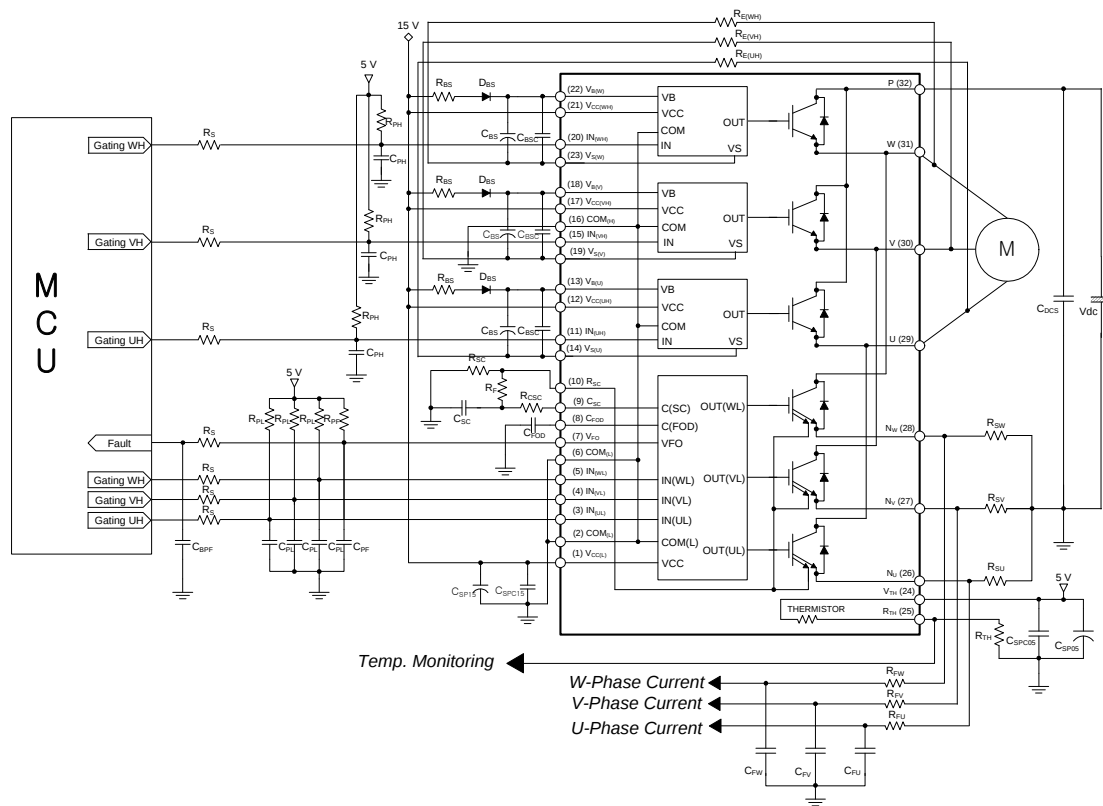
Figure 14. Application Circuit
