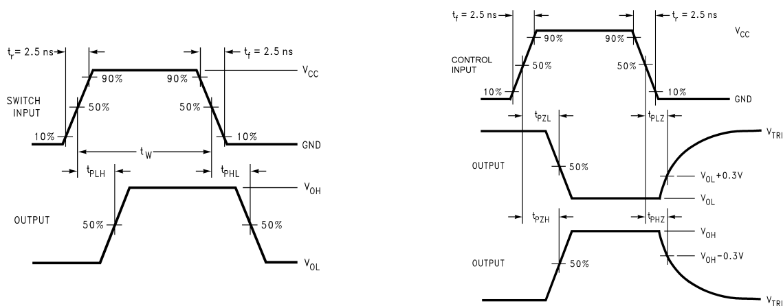
FIGURE 3. AC Waveforms
