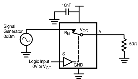
FIGURE 10. Bandwidth
