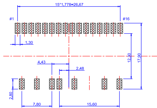
LAND PATTERN RECOMMENDATIONS
