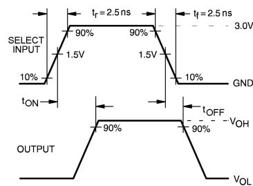
FIGURE 6. AC Waveforms
