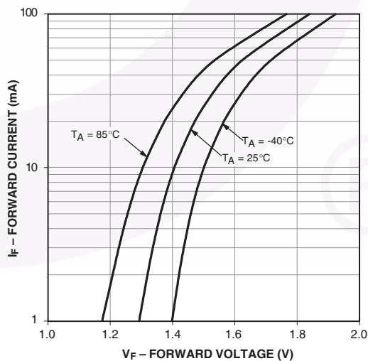
Figure 8. LED Forward Current vs. Forward Voltage
