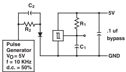
Figure 9. Switching Speed Test Circuit
