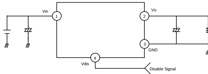
Figure 1. Application Circuit
