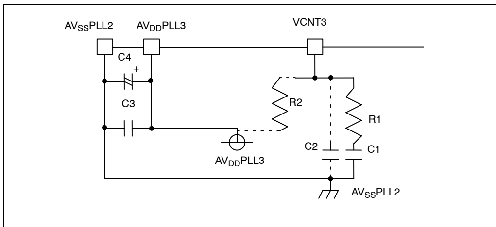
Figure 42. PLL3 (Audio)
