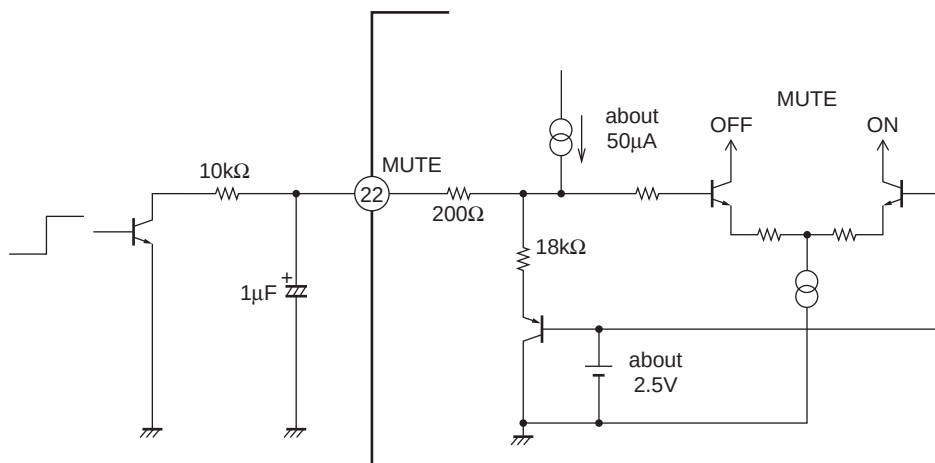
Fig2 Mute equivalent circuit
