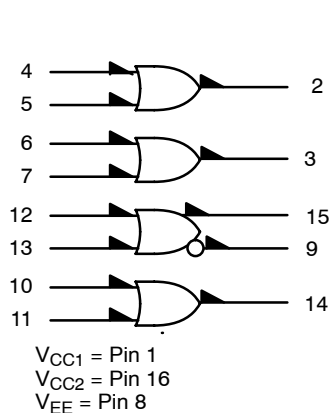
Figure 1. Logic Diagram
