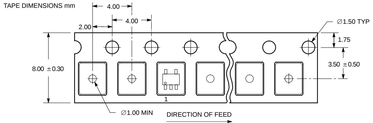
Figure 18. SC-70/SC-88A/SOT-353 DFT2 and SOT23-5/TSOP-5/SC59-5 DTT1 Reel Configuration/Orientation
