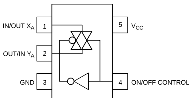
Figure 1. Pinout
